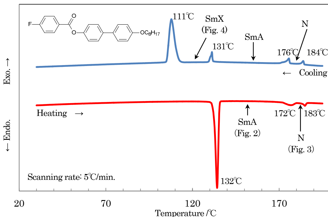
Fig.1 DSC curve of [4-(4-Ethoxyphenyl)phenyl] 4-fluorobenzoate (ID:1768)
